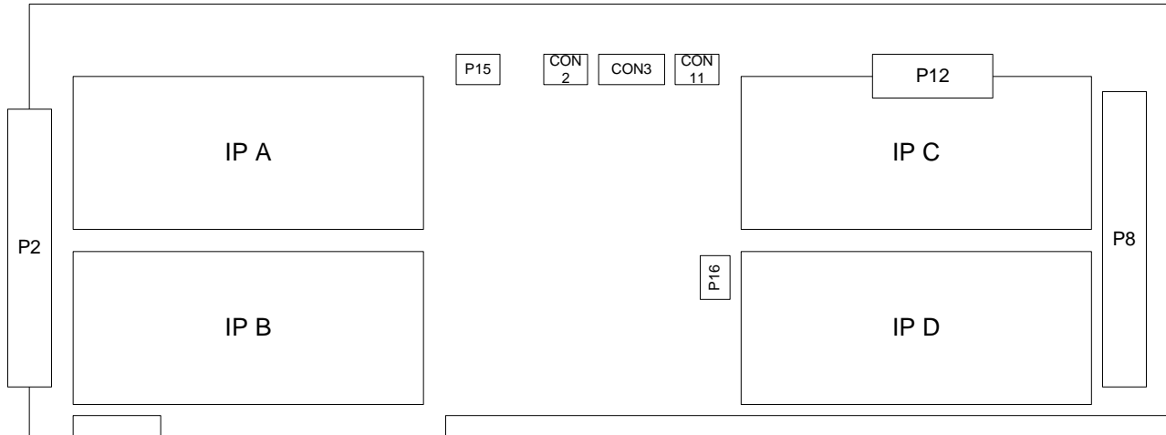
Figure 1.3: Connector Locations
