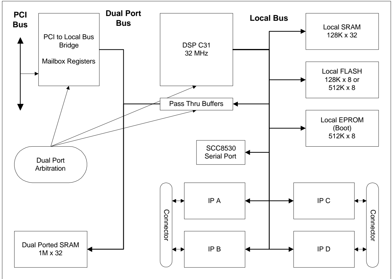
Figure 1.1: Block Diagram
