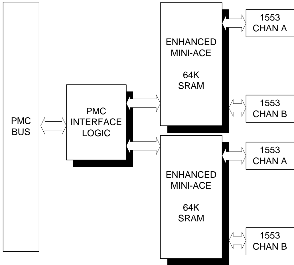
Figure 2 PMC-1553-DDC-2
