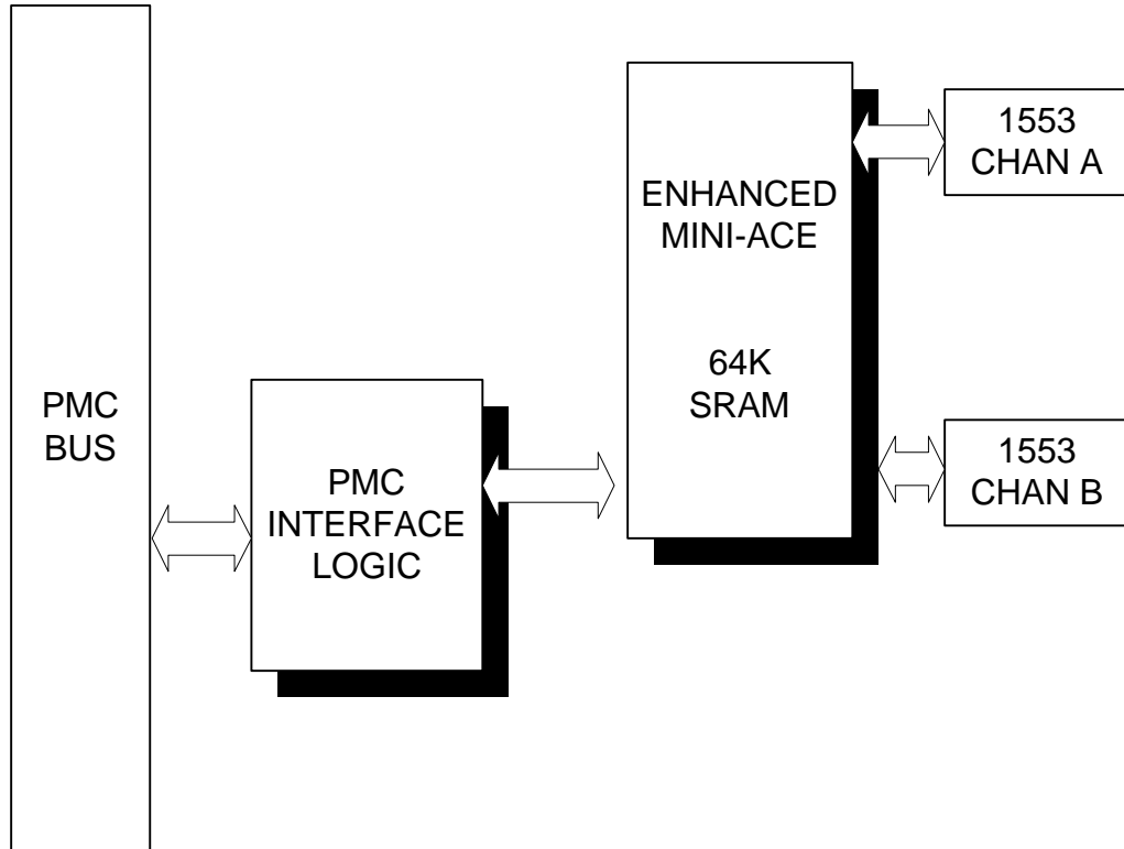
Figure 1 PMC-1553-DDC-1
