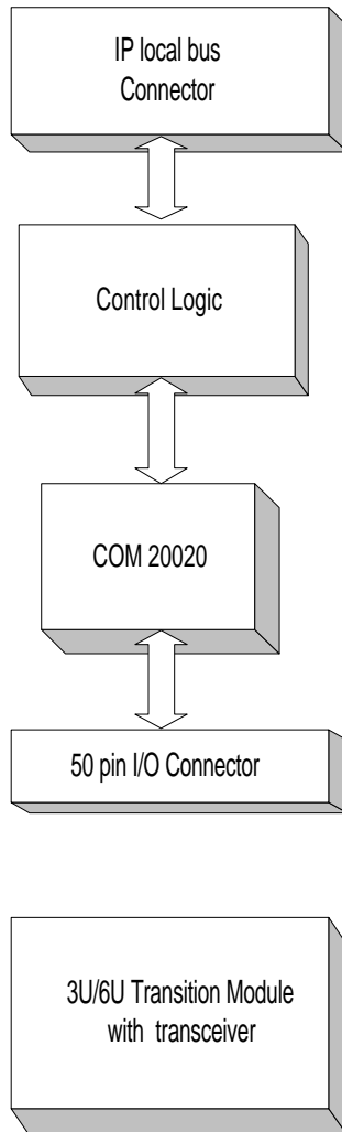
ATC-LAN1200 Functional Block Diagram
