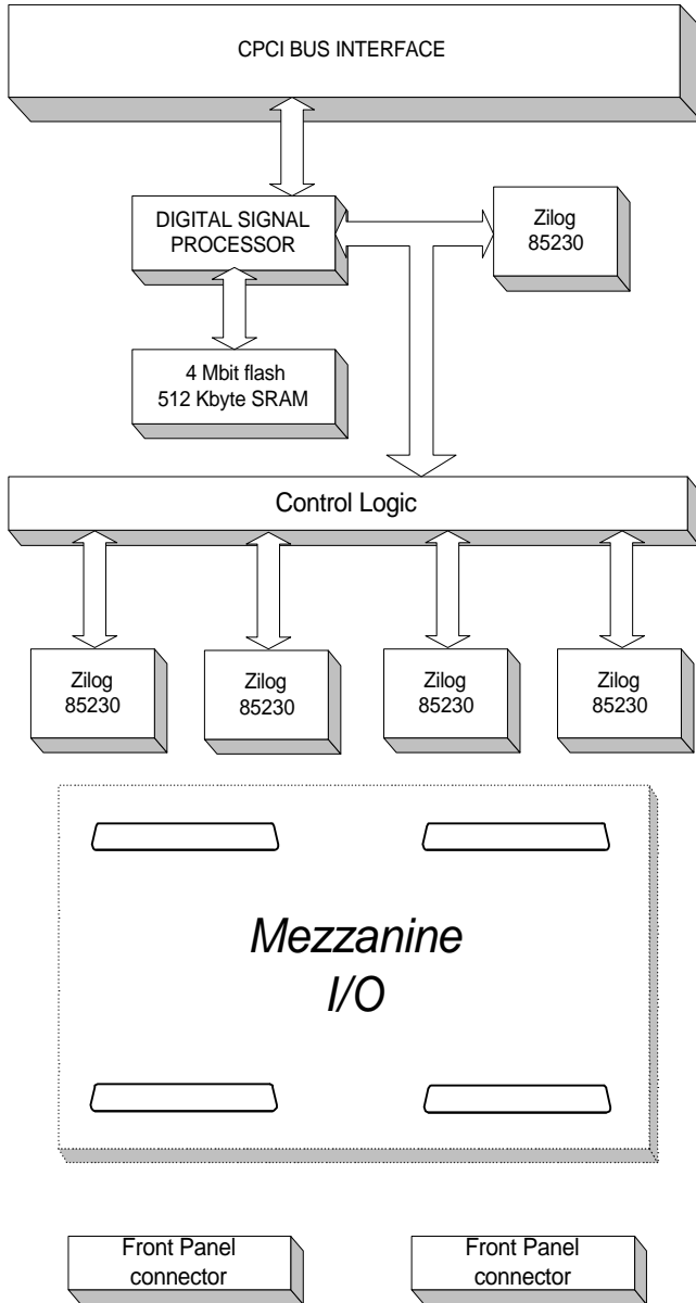
Compact PCI - Octal Serial FUNCTIONAL BLOCK DIAGRAM
