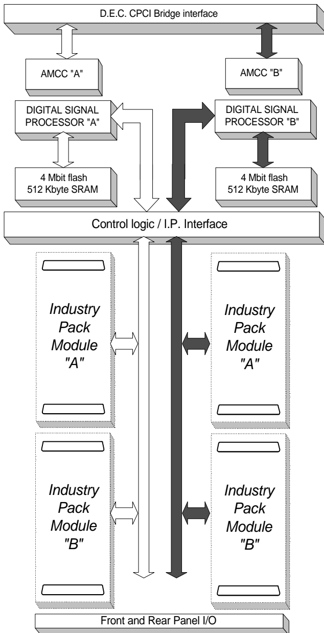
CPCI - Quad Industry Pack Carrier w/ two C31 DSP's
